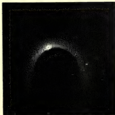
July 6.
